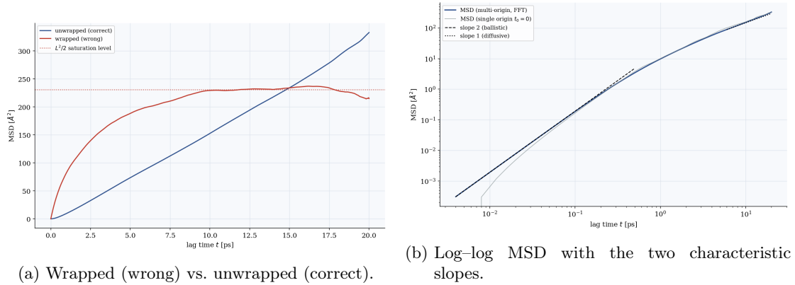
(a) Wrapped (wrong) vs. unwrapped (correct). Figure 2: (a) The wrapped MSD saturates at the geometric ceiling L^2/2 , while the unwrapped MSD grows linearly. (b) On log-log axes the unwrapped MSD shows the ballistic regime (slope 2) at short times and the diffusive regime (slope 1) at long times; the multiple-origin (FFT) estimate is far smoother than the single-origin one, especially at long lag.
