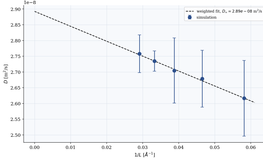
Figure 6: Self-diffusion coefficient vs. inverse box length 1/L at fixed \rho^* = 0.5 , T = 300 K (NVE production, error bars over independent seeds). The linear Yeh–Hummer trend extrapolates to the infinite-system value D_\infty at 1/L \rightarrow 0 .
